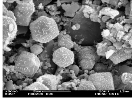
Fig. 3. C_{12}A_7 crystals with a cubic morphology and several microcrystals that have precipitated onto their surface (800 °C).
