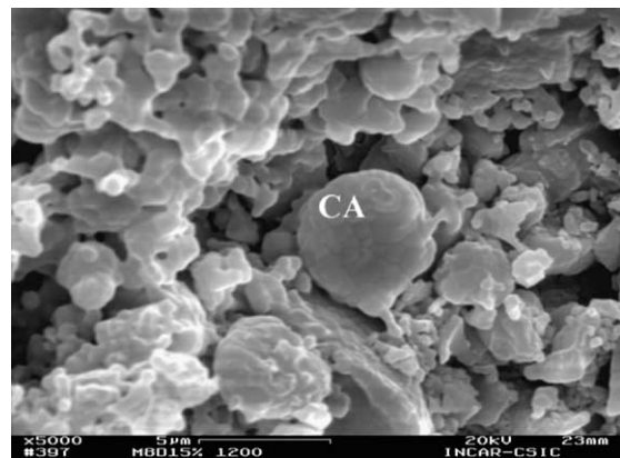
Fig. 4. CA crystal with a globular morphology (1200 °C).
